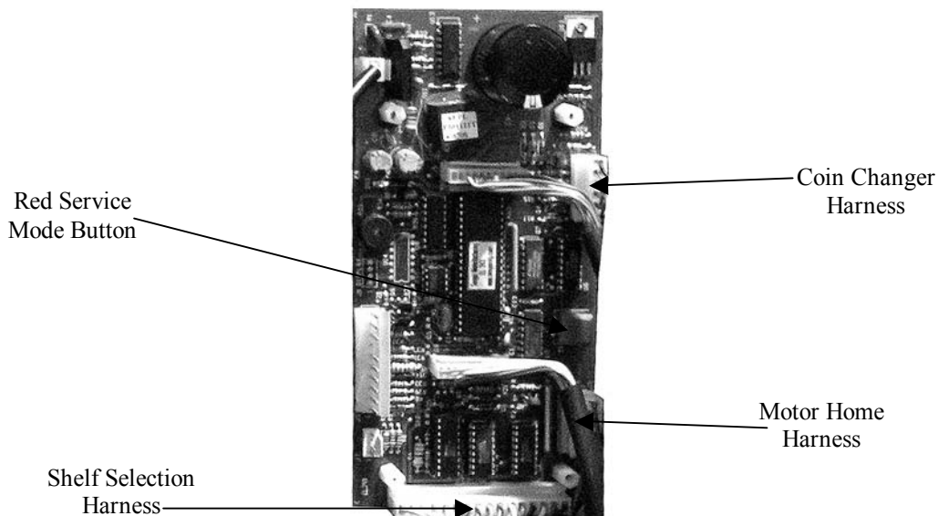
Fig. 6 – VMC Controller
