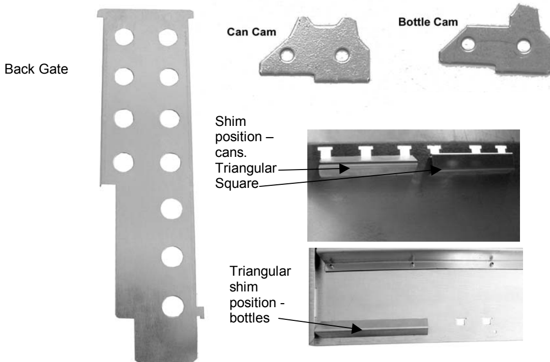
Fig. 20 Product Chute Parts
